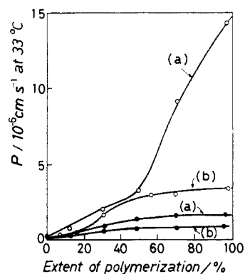
Figure 2. Effect of polymerization on permeation of NaCl (O) and the large NS 2- dye (●) from the capsule corked with 1 at 33 °C. Lipids were polymerized at (a) 5 °C and (b) 50 °C on the capsule membrane under photoirradiation for 0–20 min. The extent of polymerization was controlled by the irradiation time of the UV light and determined from the extracted monomers.
