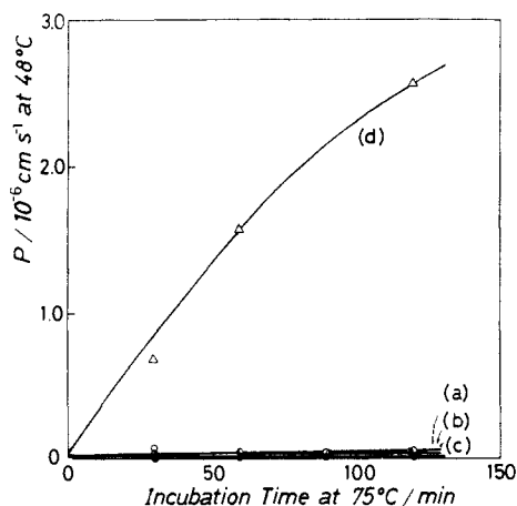
Figure 7. NaCl permeation from the capsule at 48 °C after incubation in hot water at 75 °C: (a) capsule corked with 5 and then polymerized (method A); (b) capsule corked with prepolymerized 5 (method B); (c) capsule corked with dioctadecyldimethylammonium bromide and then encased with poly(styrenesulfonate) (method C); (d) capsule corked with monomeric 5.
